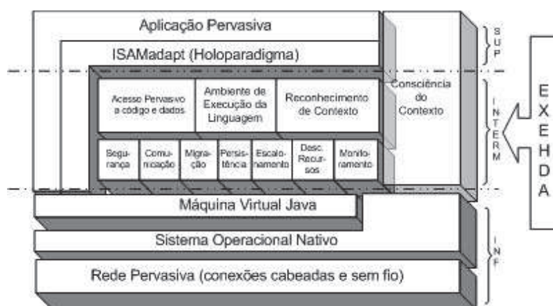
Figura 2.1: Middleware EXEHDA (YAMIN, 2004)
